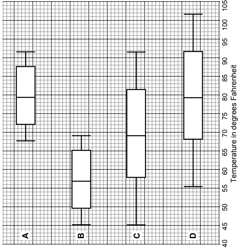
Box and whisker temperature diagrams
